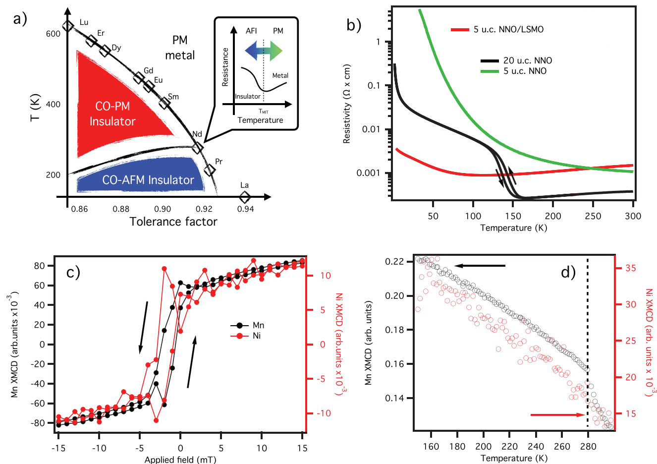
Figure 1. a) RENiO 3 phase diagram. The inset qualitatively depicts how MIT is shifted via the proximity to the magnetic orderings. b) Temperature-dependent resistivity data on NdNiO 3 systems. The bulk-like 20 u.c. NNO/NGO (black line) reference system undergoes a metal–insulator transition at 150 K. The second reference system, 5 u.c. NNO/NGO (green line), exhibits insulating behavior through the whole investigated temperature range. The 5 u.c. NNO/LSMO/NGO resistivity data show a softened MIT (red line). c) Magnetization loops measured by XMCD on the 5 u.c. NNO/LSMO/NGO sample on the Mn (black lines) and Ni (red lines) edges at 25 K. Their magnetization is in phase, indicating ferromagnetic coupling between the two layers. The magnetization curve is not centered around zero due to the flux trapped in the superconducting coils. d) Temperature dependence of Mn magnetization (black lines) and Ni (red lines) in the 5 u.c. NNO/LSMO/NGO sample under 6.5 T magnetic field: quenching of the FM ordering in LSMO above its T_C results in the same quenching in NNO.
